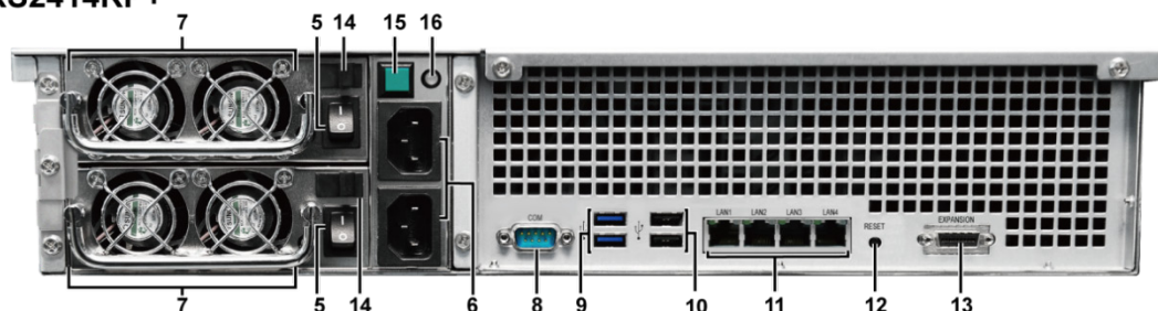
RS2414RP+
