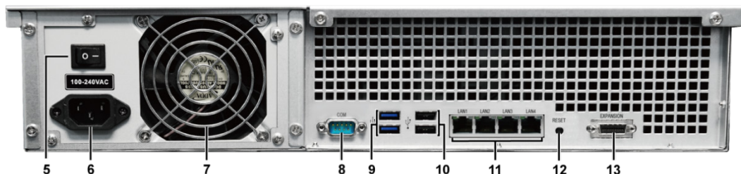
RS2414RP+
